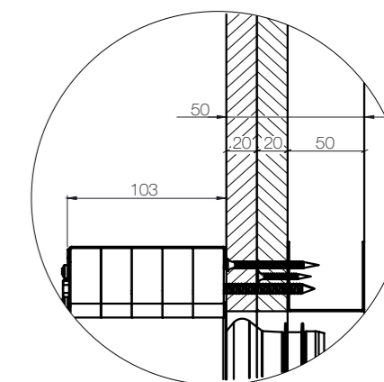
FDC25, FDC40 - stranski prerez
